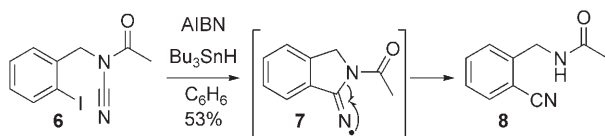
Scheme 1. 5- exo -dig cyclization of substrate 6 .
